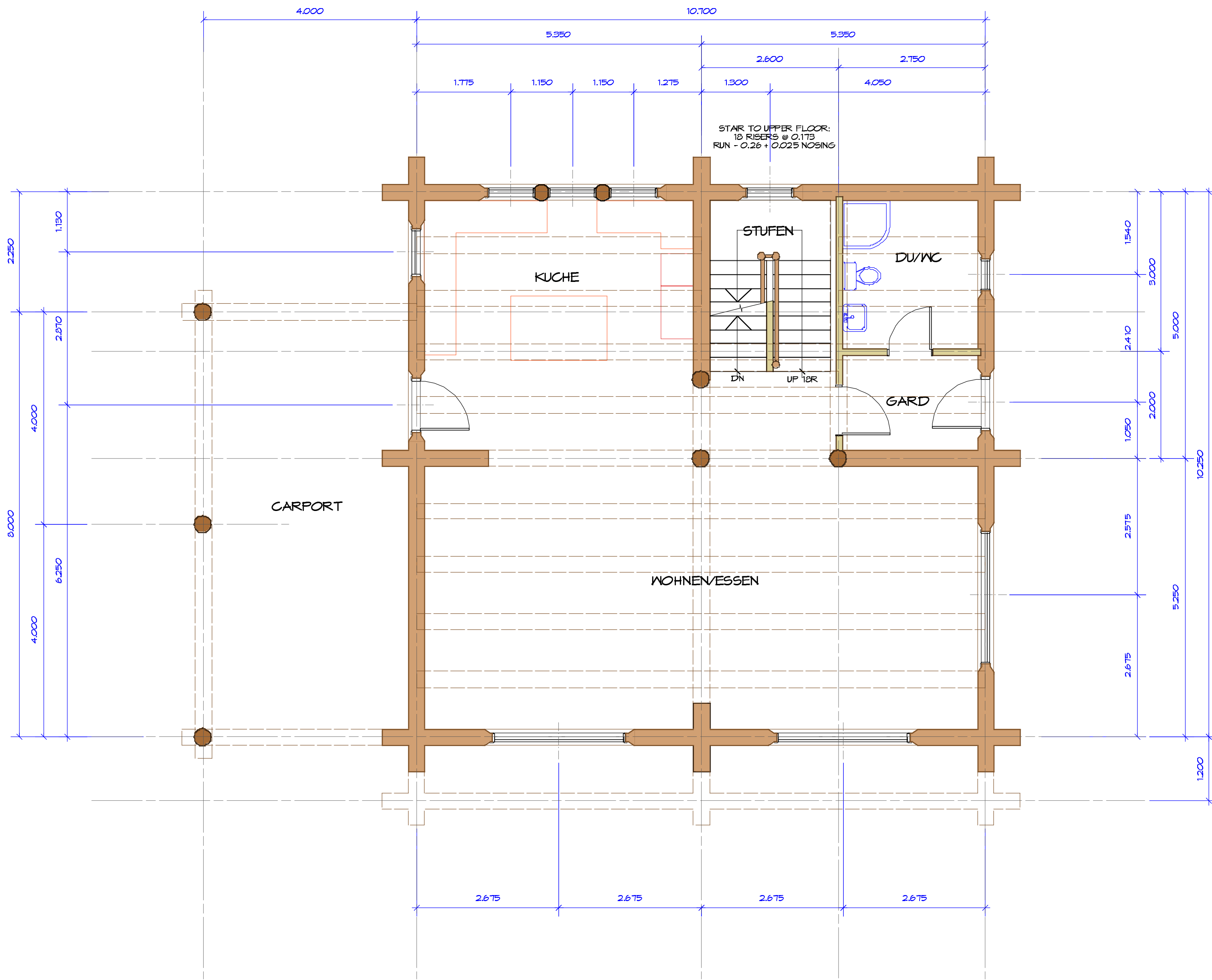
MAIN FLOOR PLAN SCALE 1:50
