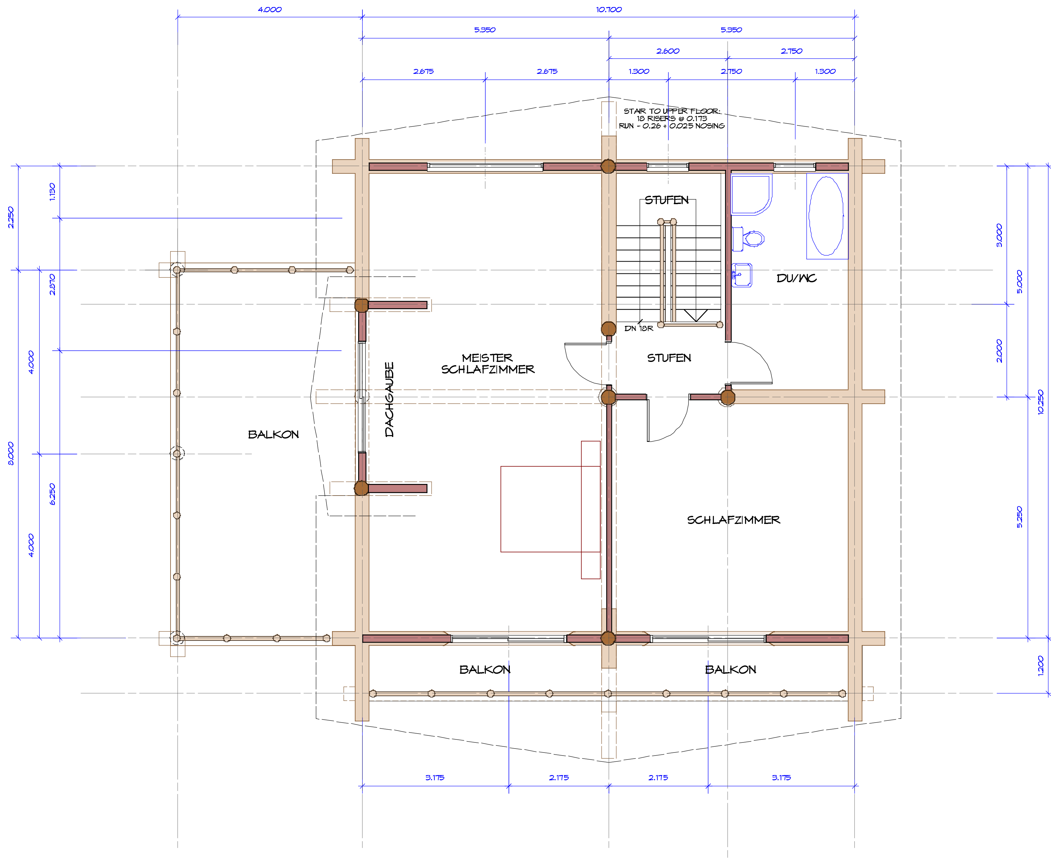
UPPER FLOOR PLAN SCALE 1/4" = 1'-0"
