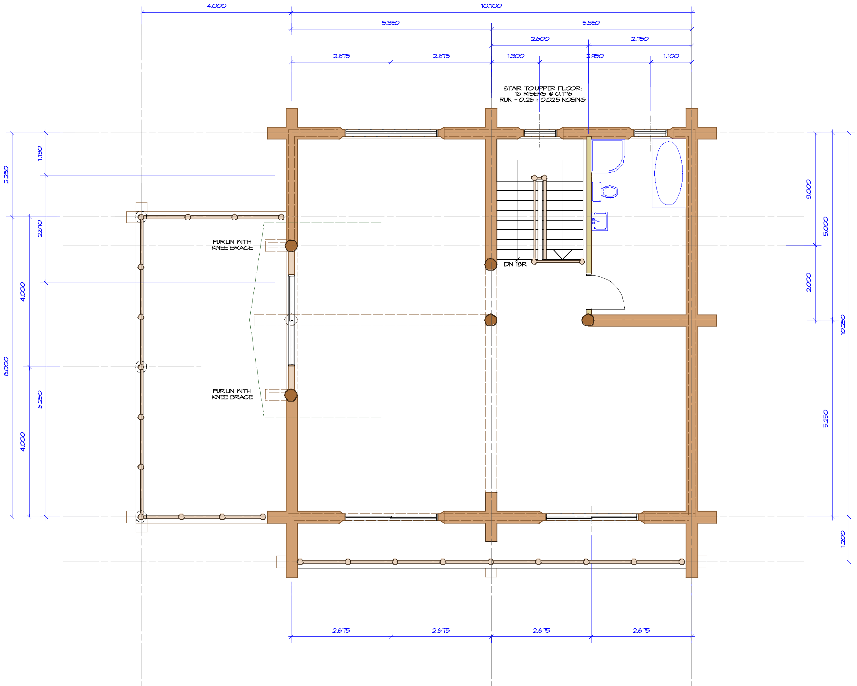
MAIN FLOOR PLAN SCALE: 1/4" = 1'-0"
